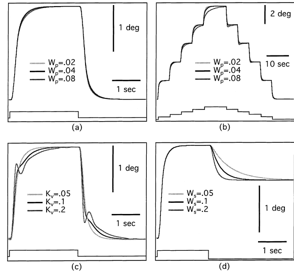
FIGURE 15. Effect of parametric variations on simulated vergence responses. The parameters specified here are described in Appendix B. (a) Closed-loop 2-deg step response under various synaptic gains at the position cells. The synaptic weights between the velocity and position cells were set as follows:
